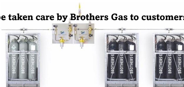
Oxygen Rack - 1x16 Cylinder (160Nm3) - 99.5%
